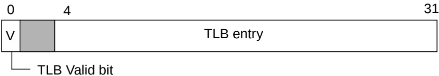
I/O TLB entry format
