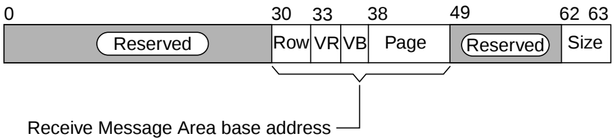
EMAC Message Reception Area Configuration register definition
