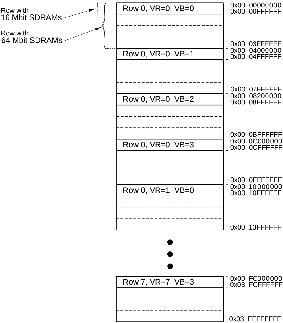
Figure 5 Coherent memory space layout
