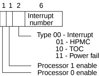
Figure 37 EPAC interrupt delivery information
