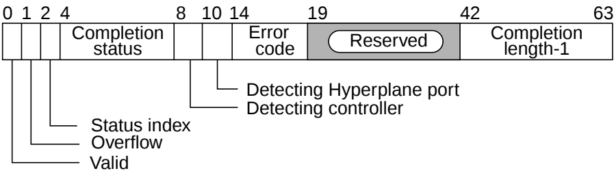
Figure 26 Operation Status Queue register definition
