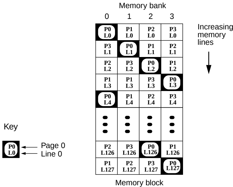
Figure 8 Single memory block interleave pattern
