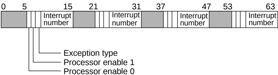
Figure 38 EPAC Interrupt Delivery register definition
