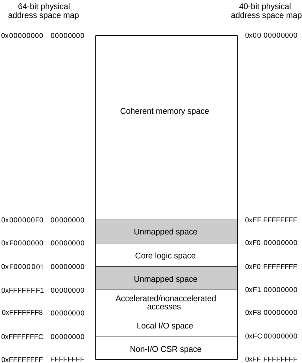
Figure 3 Physical address space partitioning
