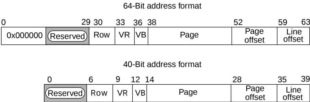
Figure 4 Coherent memory space address formats
