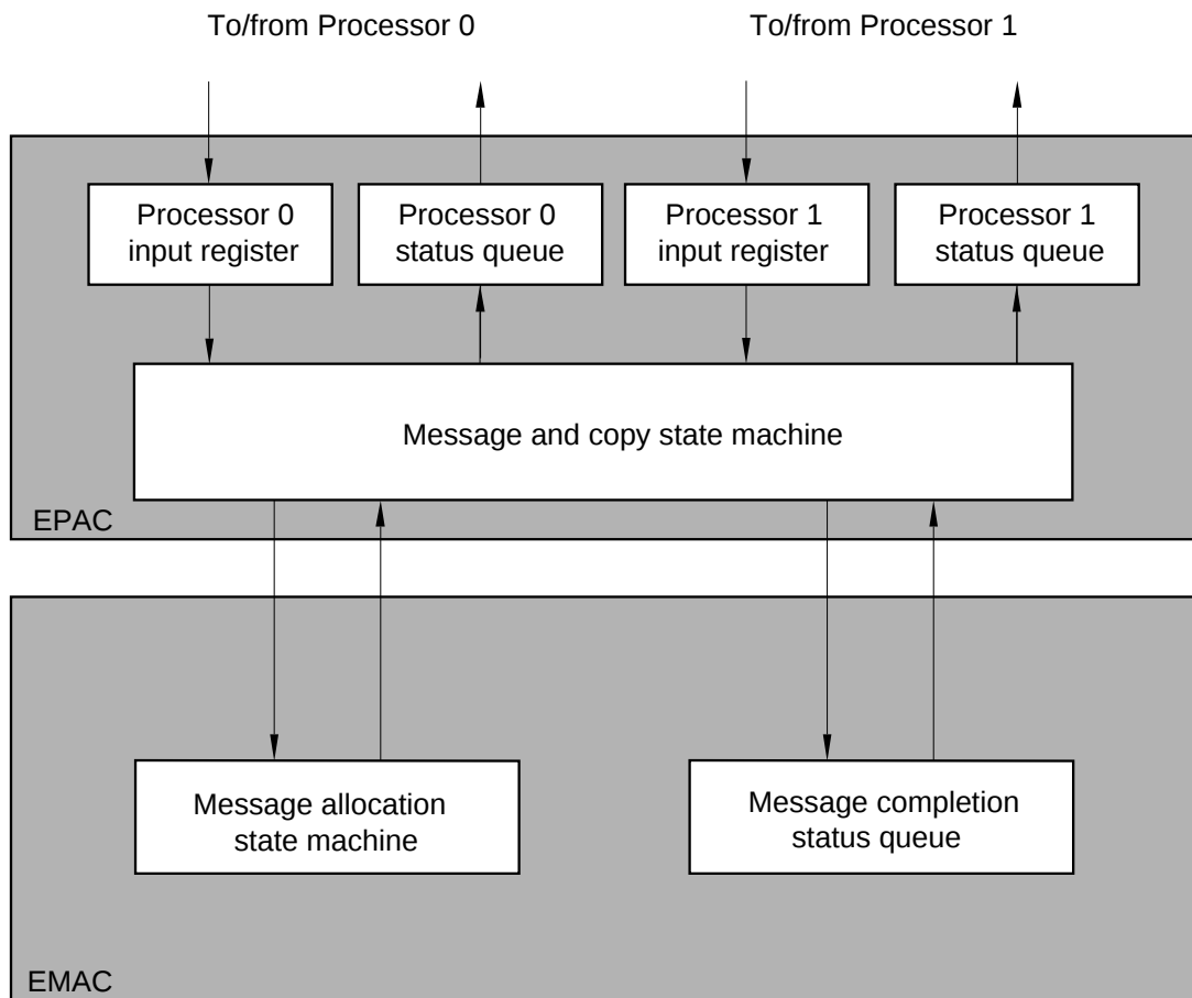
Figure 20 Messaging and data copy transfers implementation
