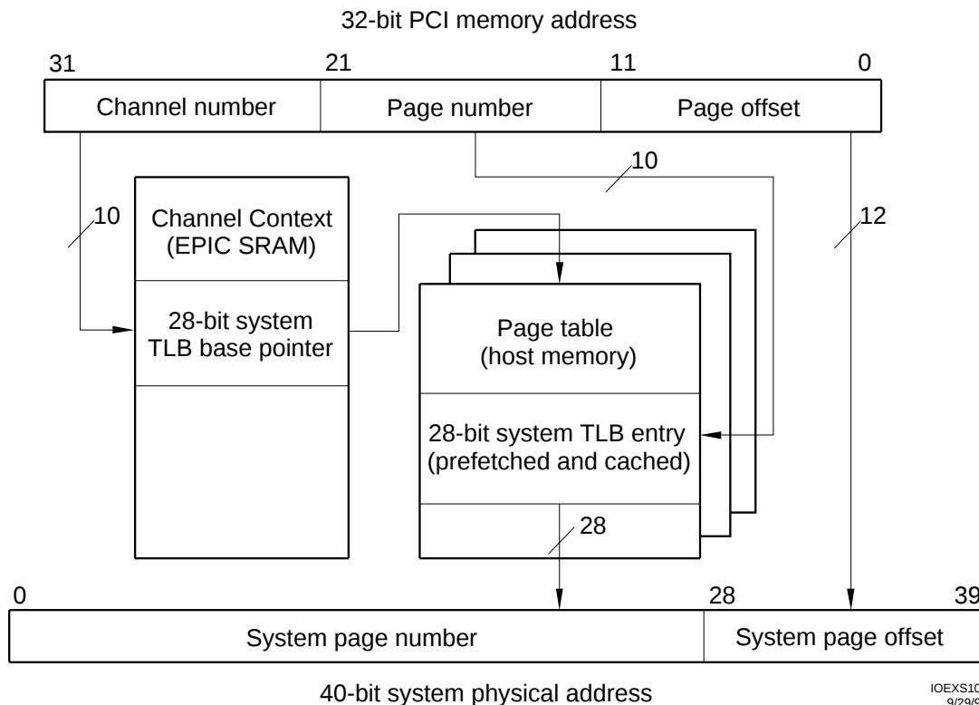
Figure 50 Logical mode address translation
