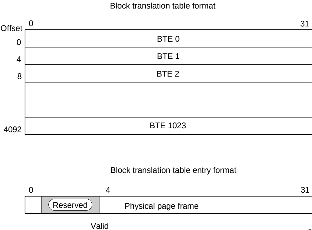
Figure 34 Block Translation Table and Entry definition
