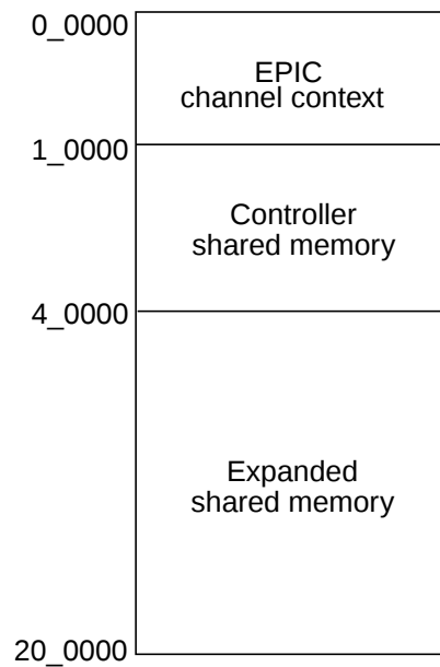
Figure 45 CCSRAM Layout
