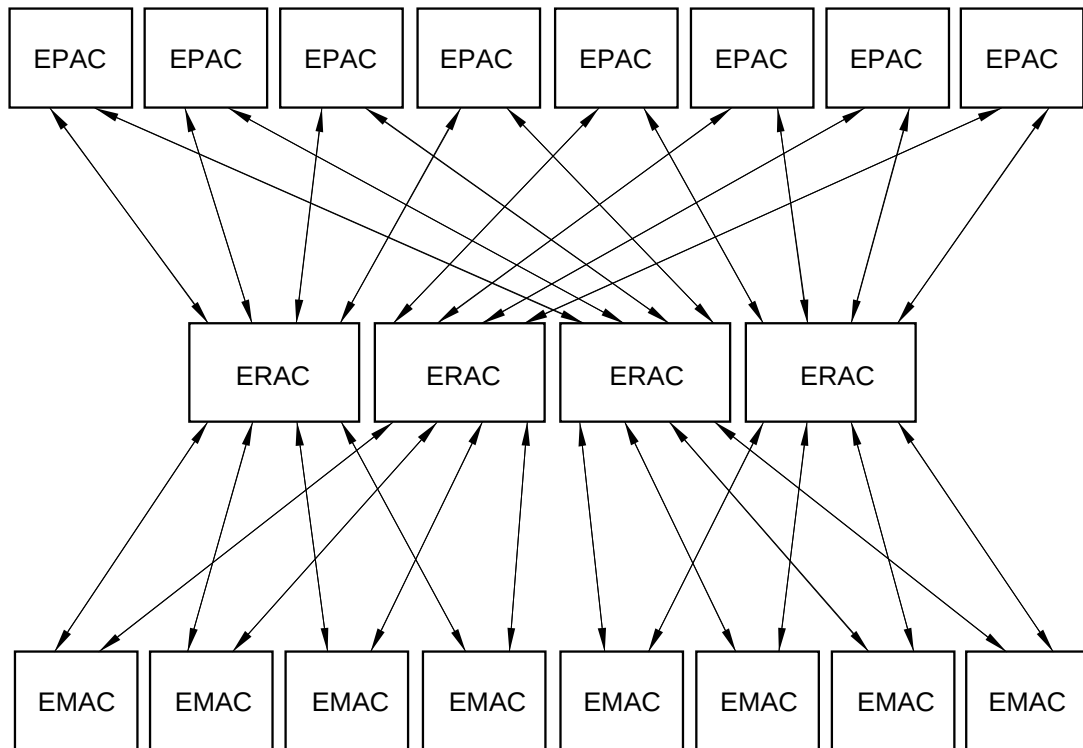
Figure 2 ERAC interconnection
